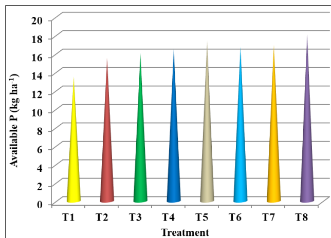
Fig 2: Available Phosphorus
