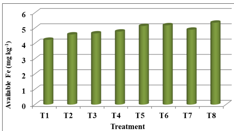
Fig 5: Available Fe
