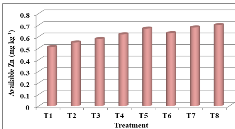
Fig 4: Available Zn
