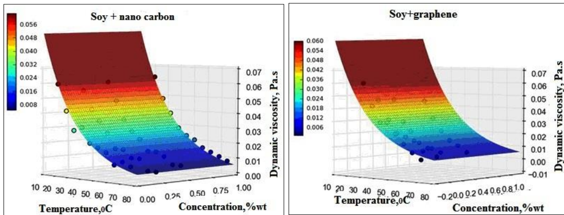
Fig 1: 3D representation of the mathematical function of the dependence of dynamic viscosity on temperature and additive concentration
